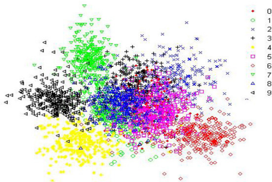
Figure 1: Two-dimensional embedding of 3,000 USPS test data points using MCML.
